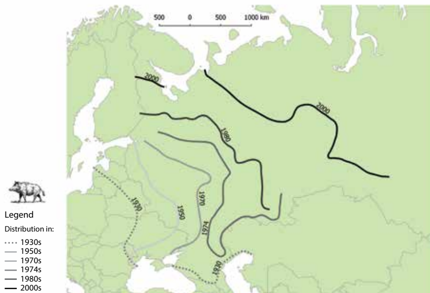
FIGURE 8 Changes in wild boar distribution range in the ex-USSR
